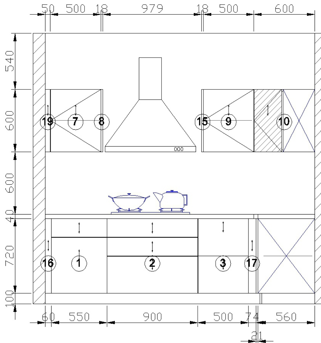
B View elevation drawing
