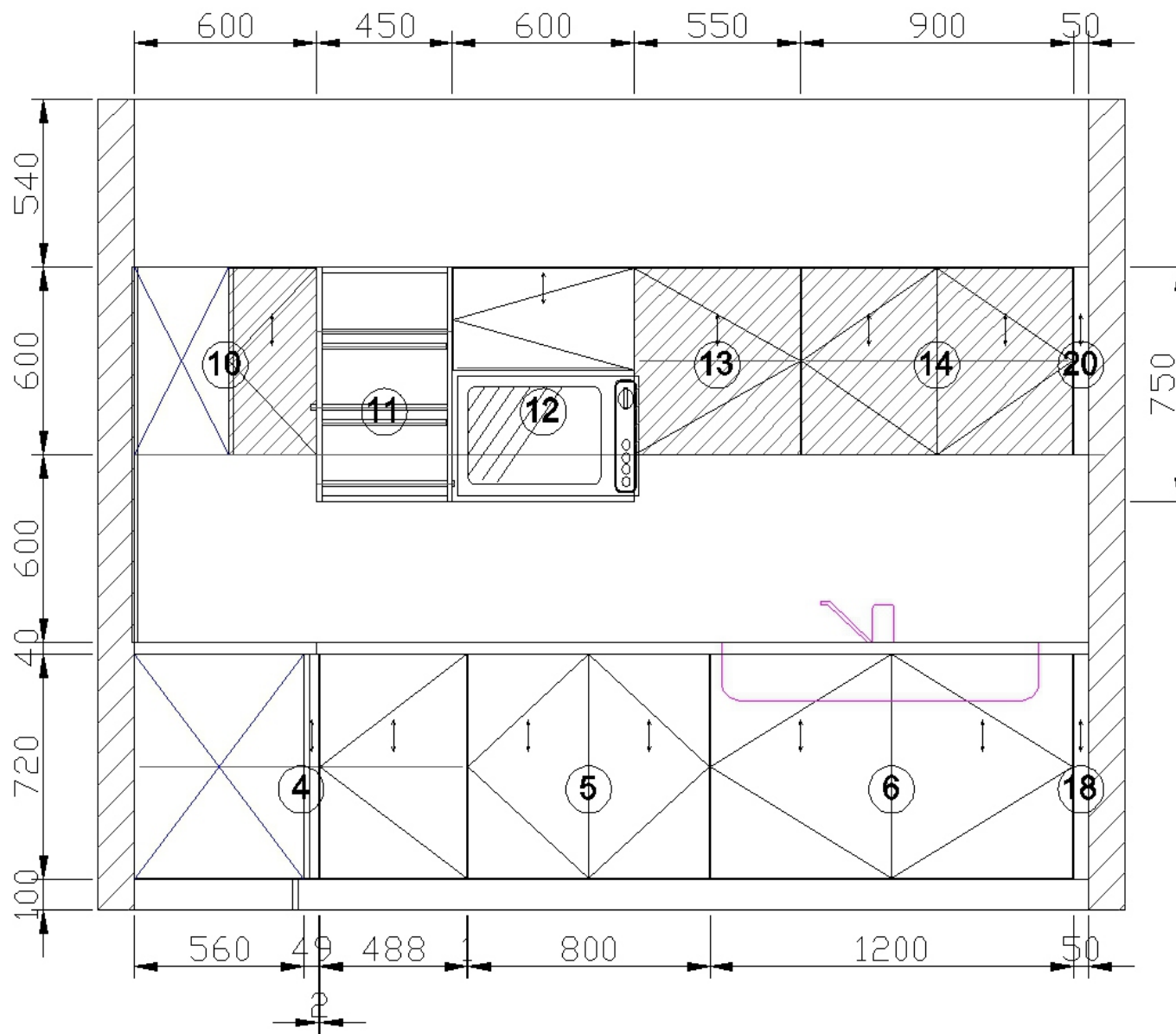
A View elevation drawing
